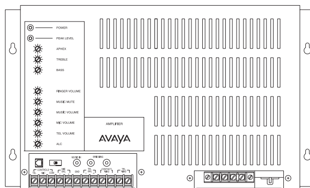
Figure 1: Telephone Paging Amplifier
